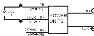
120V TAP CONNECTION
