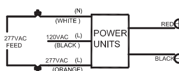
277V TAP CONNECTION
